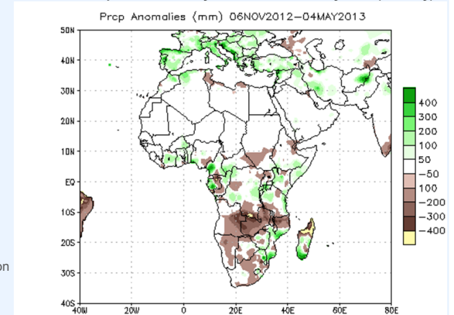
Data Source: CPC Unified (gauge-based & 0.5x0.5 deg resolution) Precipitation Analysis Climatology (1981-2010)
