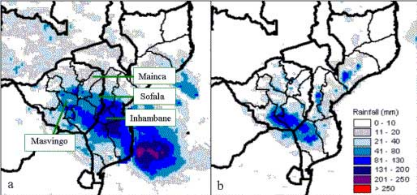
Figure 1. Japhet-induced rainfall since March 1. Figure 1.a shows the total daily rainfall from March 1 to March 4, while Figure 1.b shows the rainfall on March 5. The rainfall figures shown are based on satellite-derived rainfall estimates.
