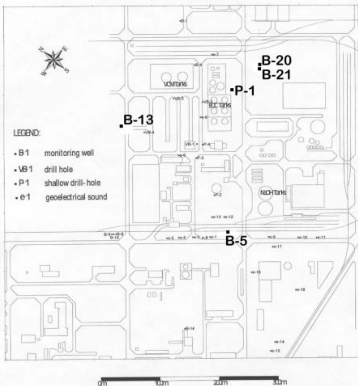
Figure 3: Locations of groundwater sampling wells at HIP Petrohemija
