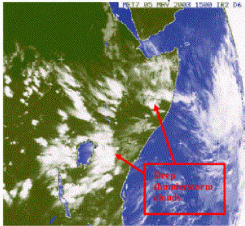
Figure 1: Major storm systems affecting the equatorial sector of the GHA – 05 May 2003
