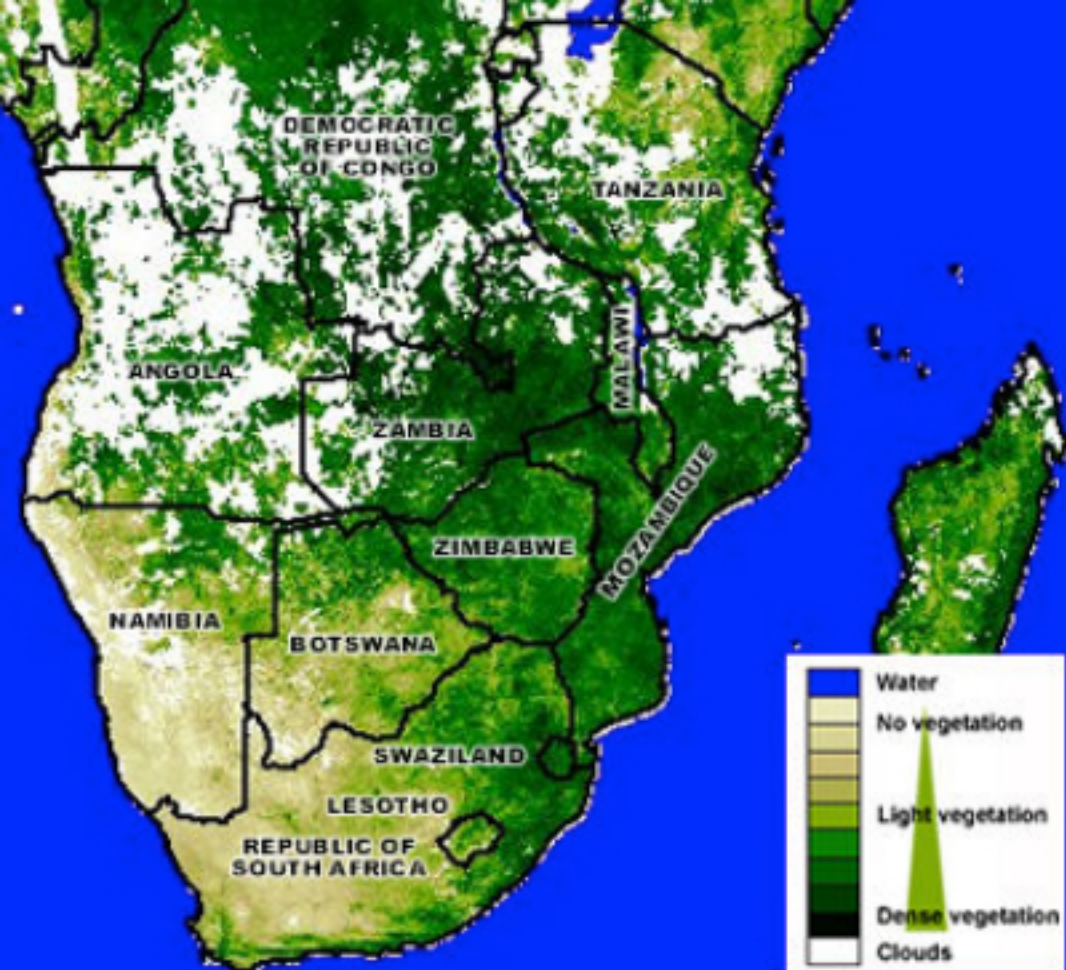
State of vegetation (NDVI) January 2004
